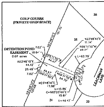
DETAIL 6 DRAINAGE EASEMENT SCALE: 1"=50'
