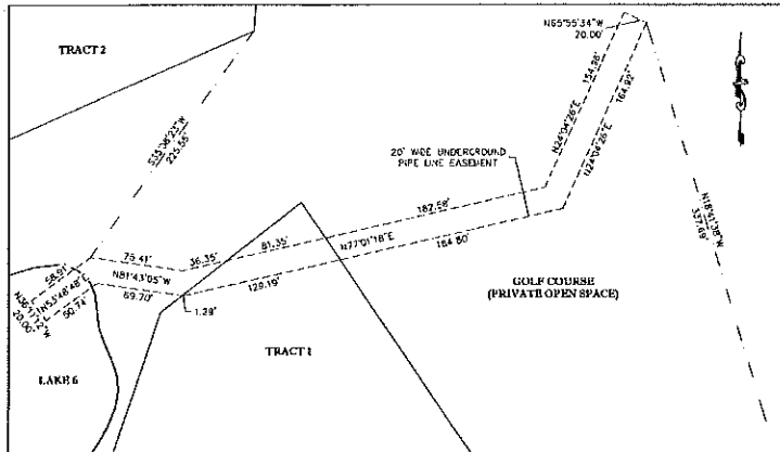
DETAIL 25 UNDERGROUND PIPE LINE EASEMENT SCALE: 1"=50'
