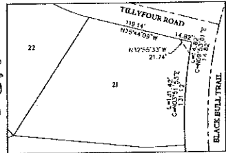
DETAIL 17 TRAIL EASEMENT SCALE: 1"=50'
