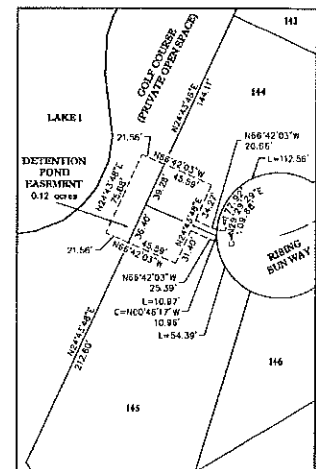
DETAIL 30 DRAINAGE EASEMENT SCALE: 1"=50'
