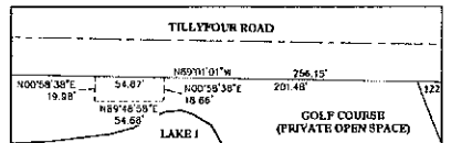
DETAIL 28 LIFT STATION EASEMENT SCALE: 1"=50'
