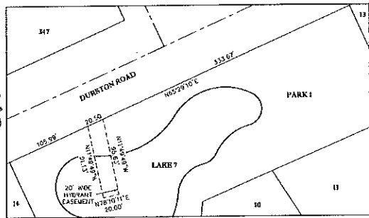
DETAIL 5 WATERLINE EASEMENT SCALE: 1"=50'
