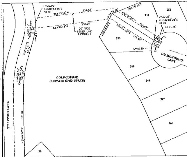
DETAIL 1 SEWERLINE EASEMENT SCALE: 1"=50'
