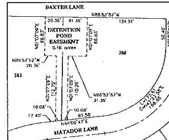
DETAIL 8 DRAINAGE EASEMENT SCALE: 1"=50'
