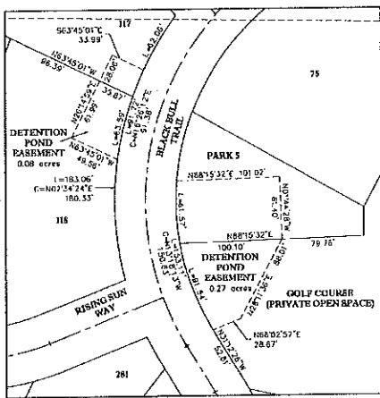
DETAIL 14 DRAINAGE EASEMENT SCALE: 1"=50'
