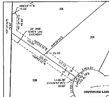
DETAIL 3 SEWERLINE EASEMENT SCALE: 1"=50'
