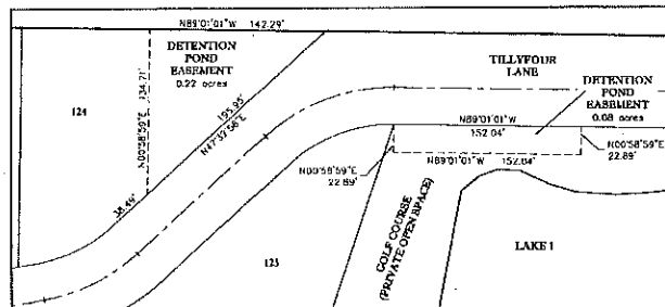
DETAIL 13 DRAINAGE EASEMENT SCALE: 1"=50'
