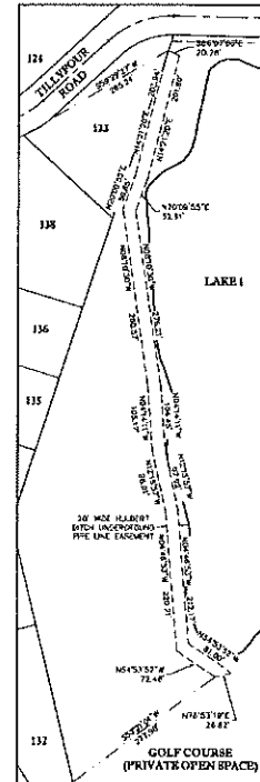
DETAIL 26 IRRIGATION DITCH EASEMENT SCALE: 1"=100'
