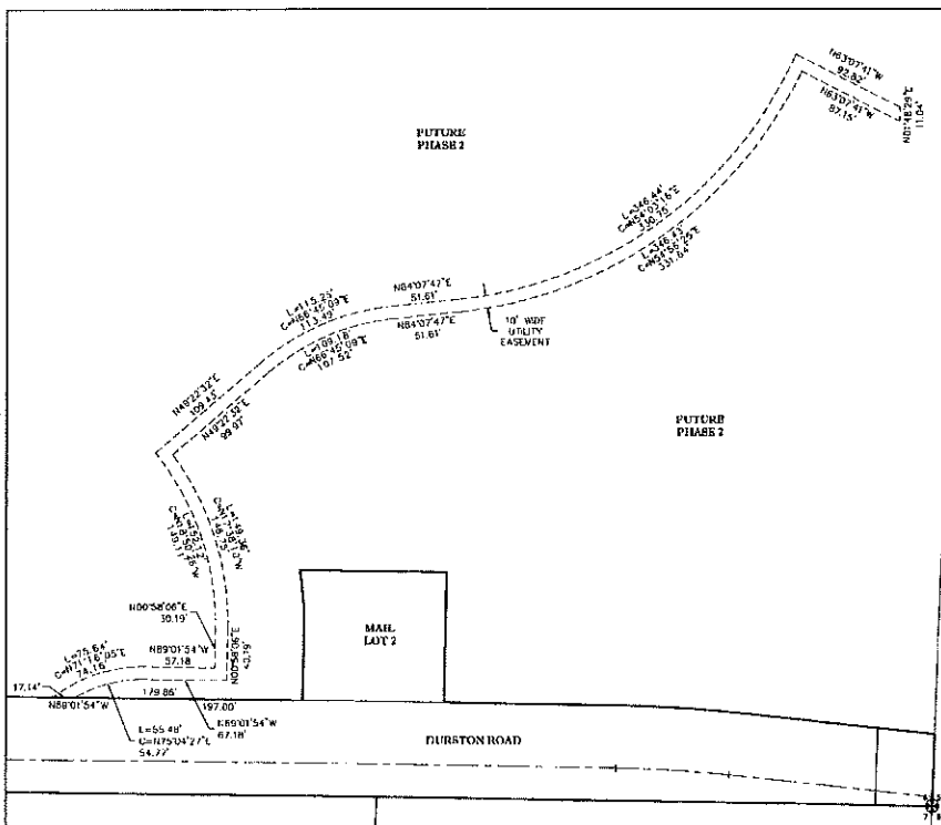
DETAIL 29 UTILITY EASEMENT SCALE: 1"=50'
