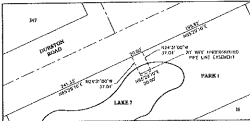
DETAIL 20 UNDERGROUND PIPE LINE EASEMENT SCALE: 1"=50'
