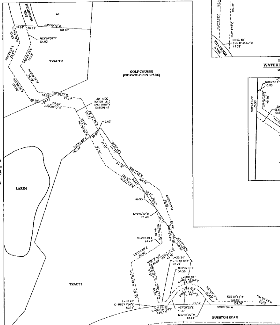
DETAIL 4 WATERLINE EASEMENT SCALE: 1"=50'
