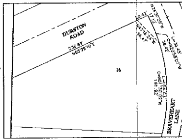
DETAIL 18 TRAIL EASEMENT SCALE: 1"=50'
