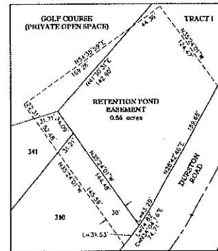
DETAIL 7 DRAINAGE EASEMENT SCALE: 1"=50'
