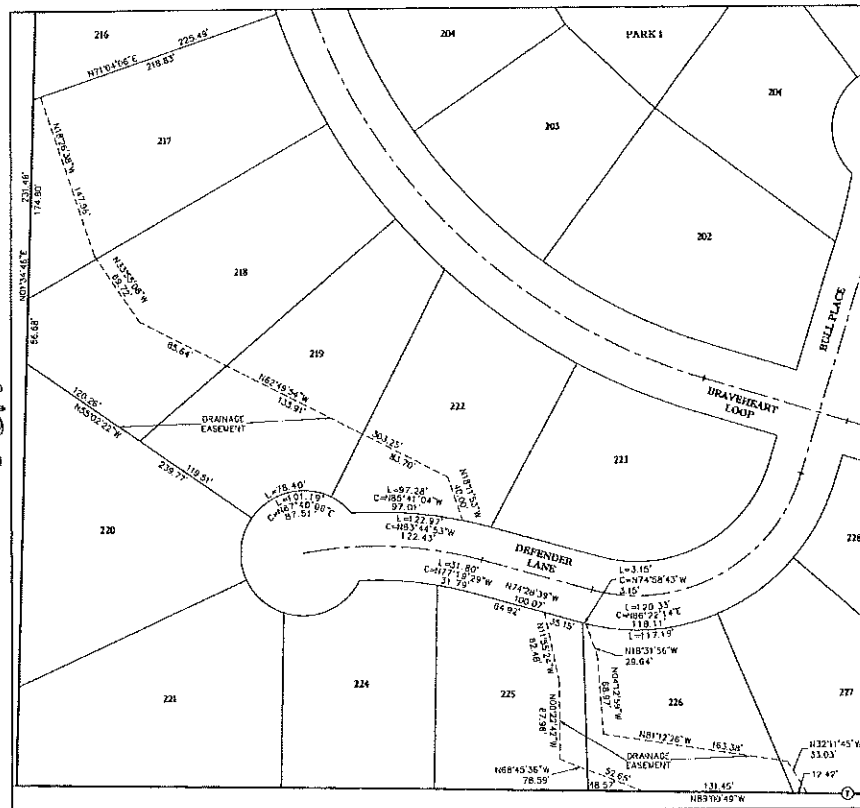
DETAIL 11 DRAINAGE EASEMENT SCALE: 1"=50'
