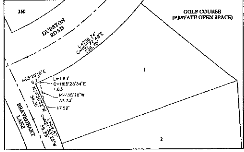
DETAIL 21 TRAIL EASEMENT SCALE: 1"=50'
