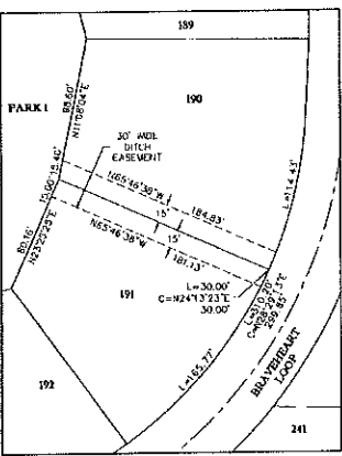
DETAIL 22 IRRIGATION DITCH EASEMENT SCALE: 1"=50'
