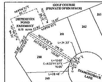
DETAIL 9 DRAINAGE EASEMENT SCALE: 1"=50'
