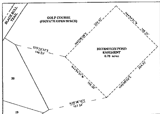
DETAIL 12 DRAINAGE EASEMENT SCALE: 1"=50'
