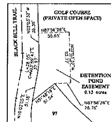
DETAIL 31 DRAINAGE EASEMENT SCALE: 1"=50'
