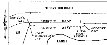
DETAIL 27 UTILITY EASEMENT SCALE: 1"=50'
