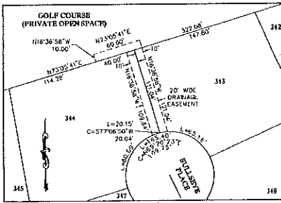
DETAIL 15 DRAINAGE EASEMENT SCALE: 1"=50'
