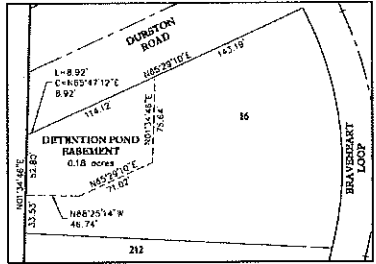
DETAIL 16 DRAINAGE EASEMENT SCALE: 1"=50'
