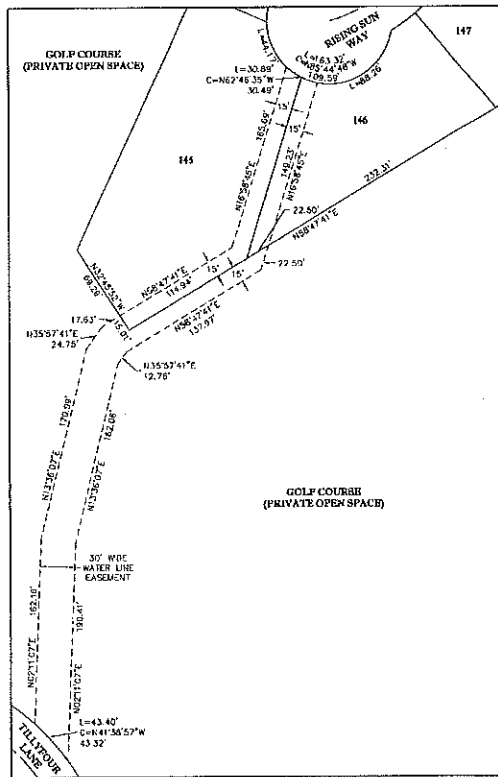
DETAIL 2 WATERLINE EASEMENT SCALE: 1"=50'
